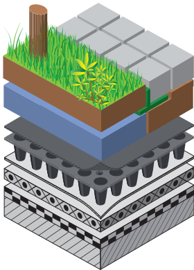
Composition Nophadrain Extensive and Intensive Green Roof
